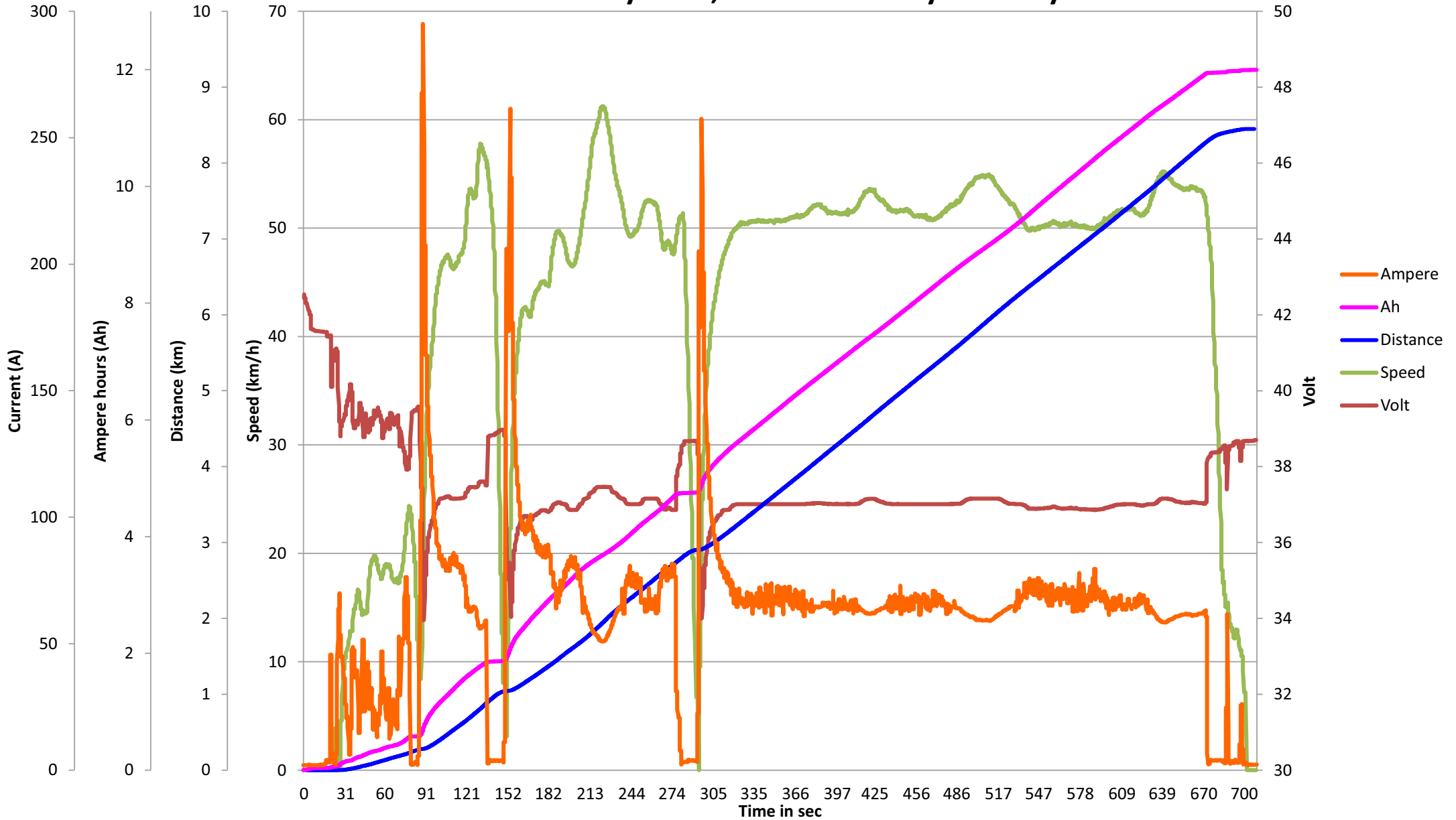
CityEL 38,4V Data from Cycle Analyst
